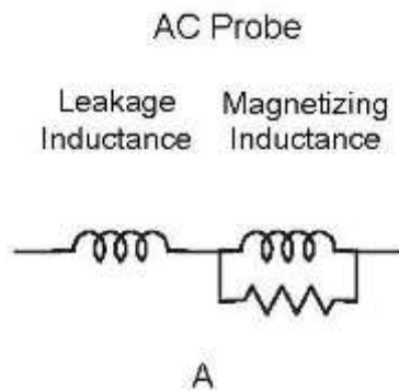
Figure 1. Insertion Impedance A
